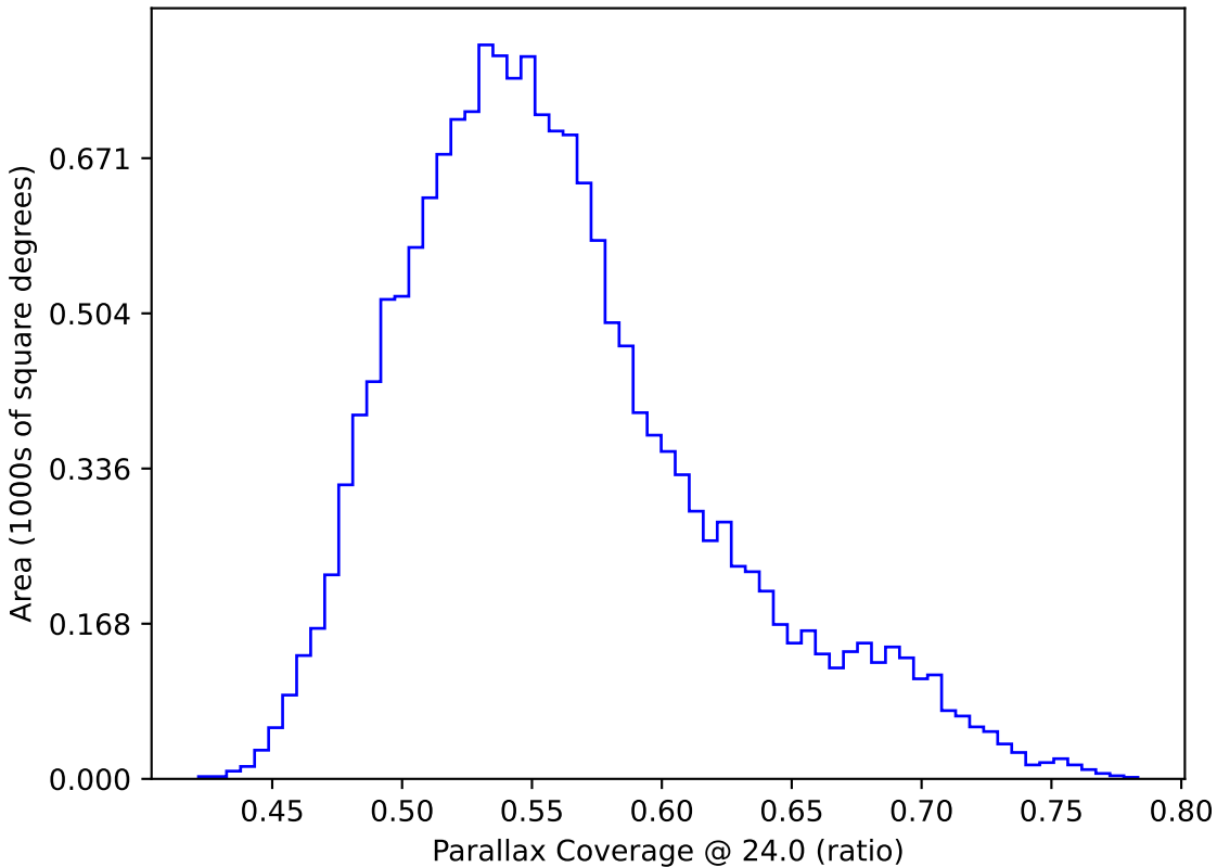
ddf_loaded_fl15_v3.4_10yrs WFD: Parallax Coverage @ 24.0
