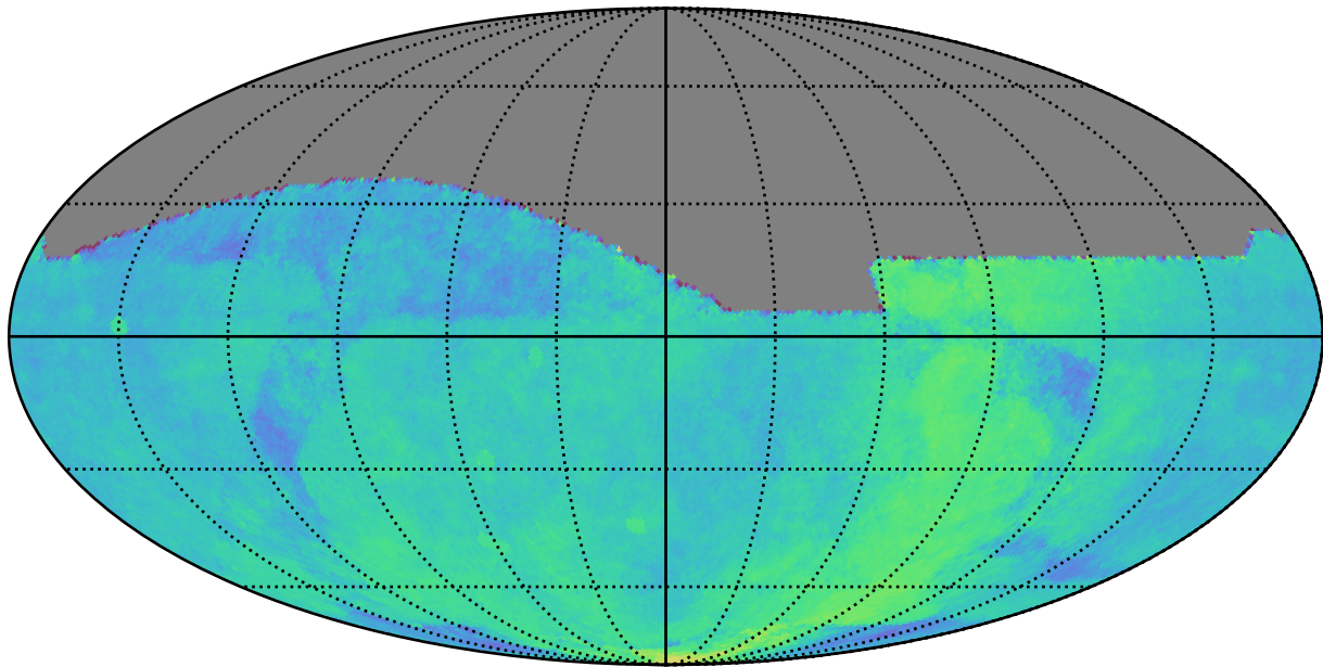
ddf_loaded_fl15_v3.4_10yrs All sky: Parallax Coverage @ 24.0
