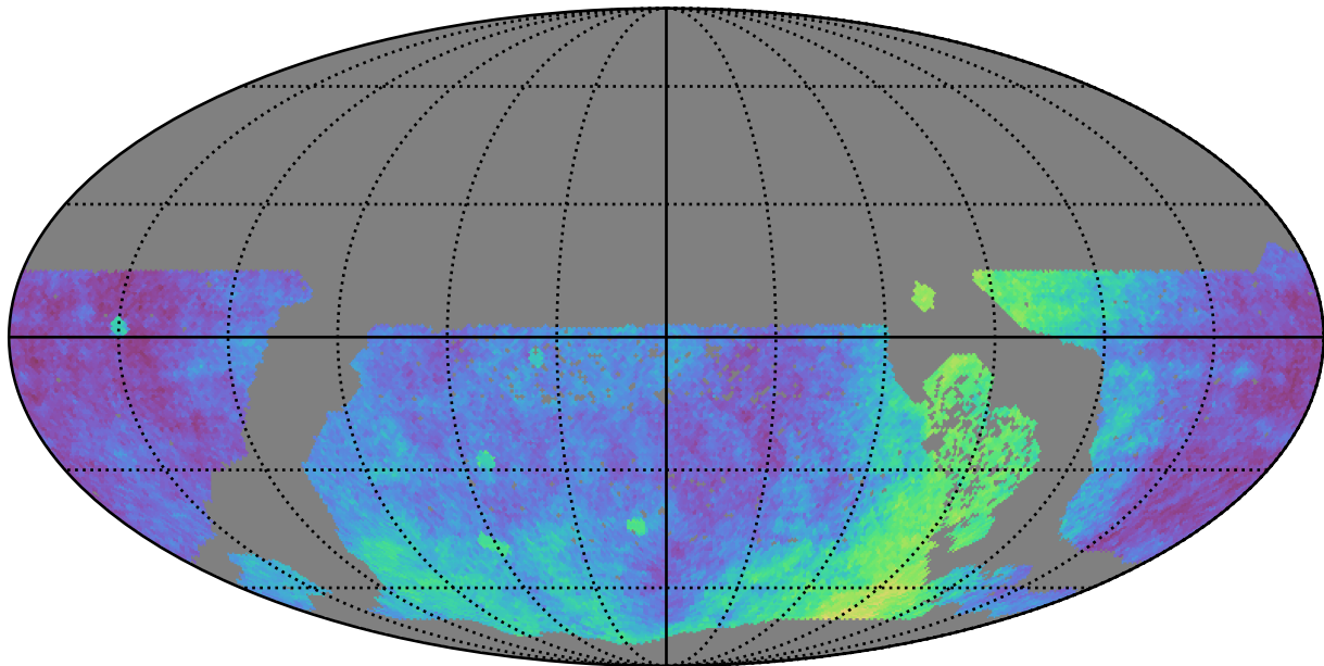
ddf_loaded_fl15_v3.4_10yrs WFD: Parallax Coverage @ 22.4
