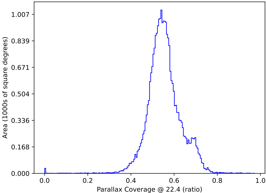
ddf_loaded_fl15_v3.4_10yrs All sky: Parallax Coverage @ 22.4
