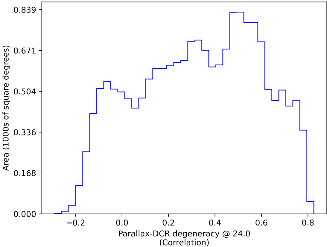
ddf_loaded_fl15_v3.4_10yrs WFD: Parallax-DCR degeneracy @ 24.0
