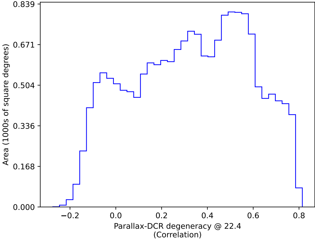
ddf_loaded_fl15_v3.4_10yrs WFD: Parallax-DCR degeneracy @ 22.4
