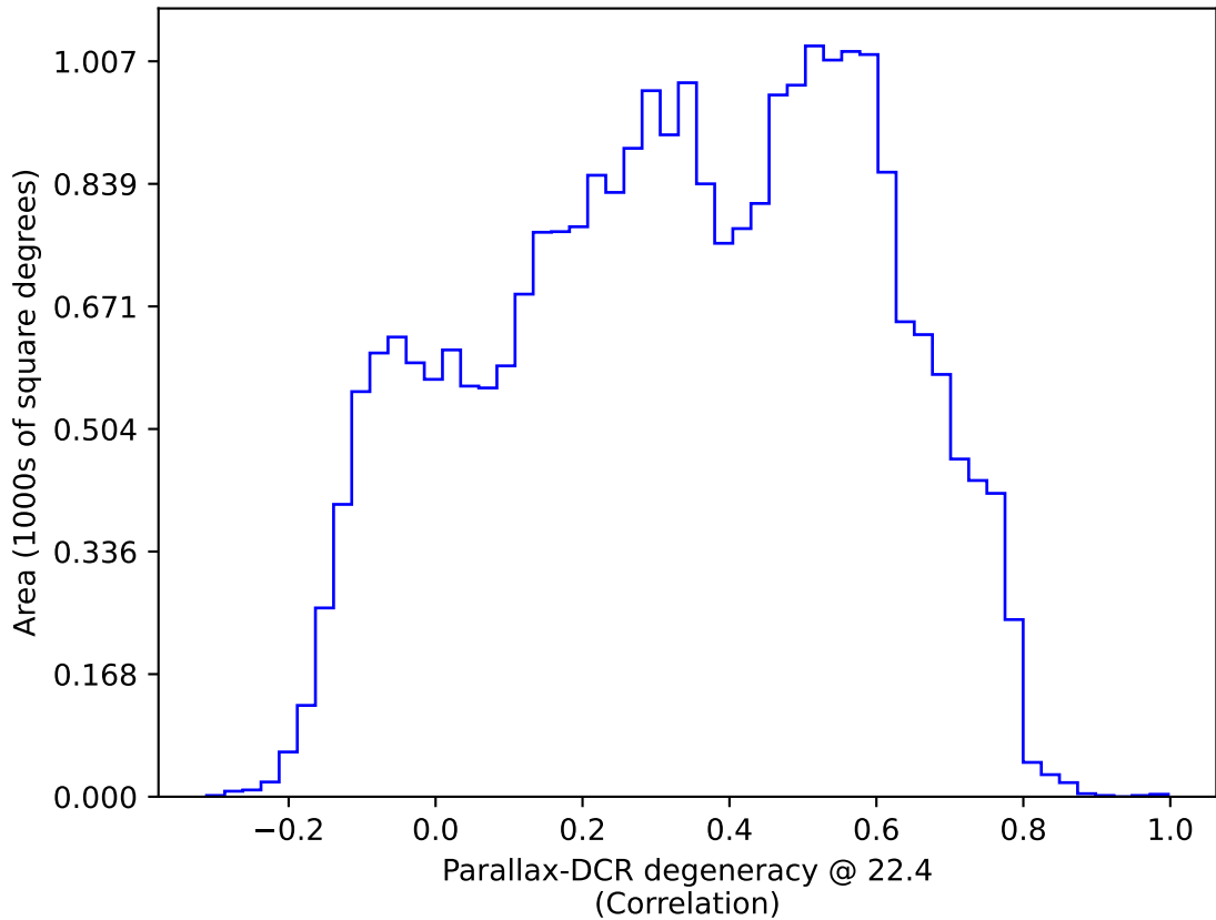
ddf_loaded_fl15_v3.4_10yrs All sky: Parallax-DCR degeneracy @ 22.4
