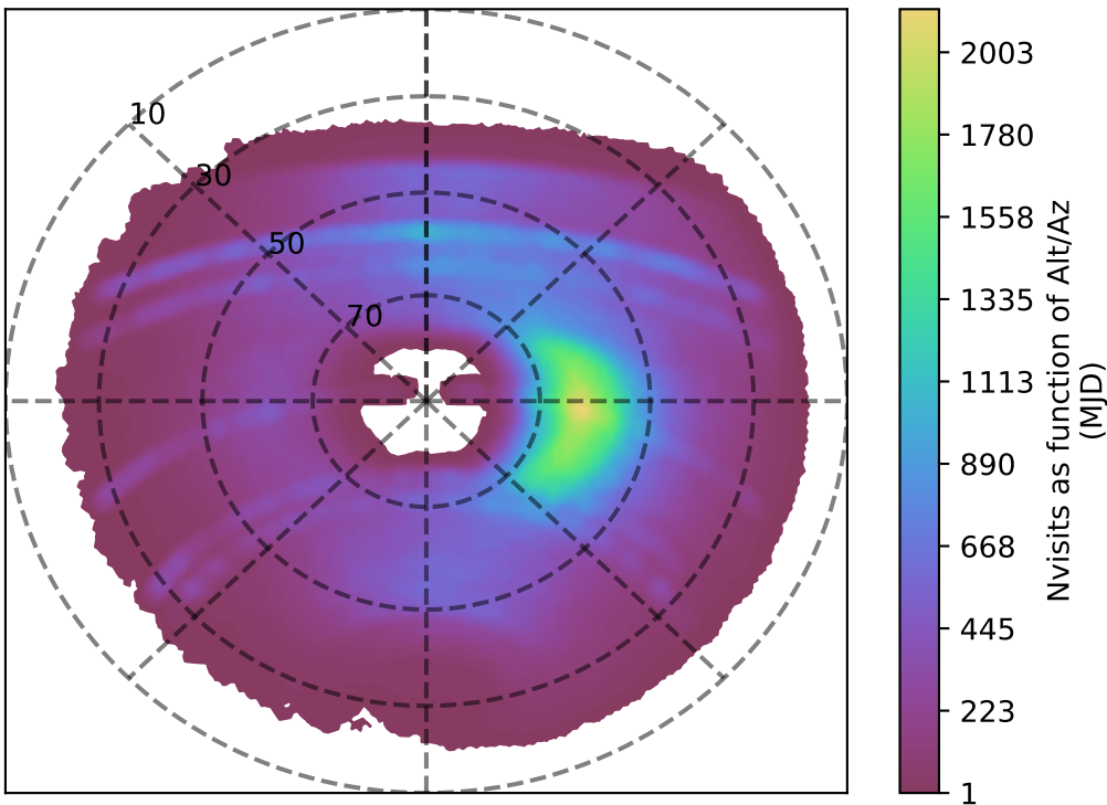
ddf_loaded_fl15_v3.4_10yrs y band: Nvisits as function of Alt/Az
