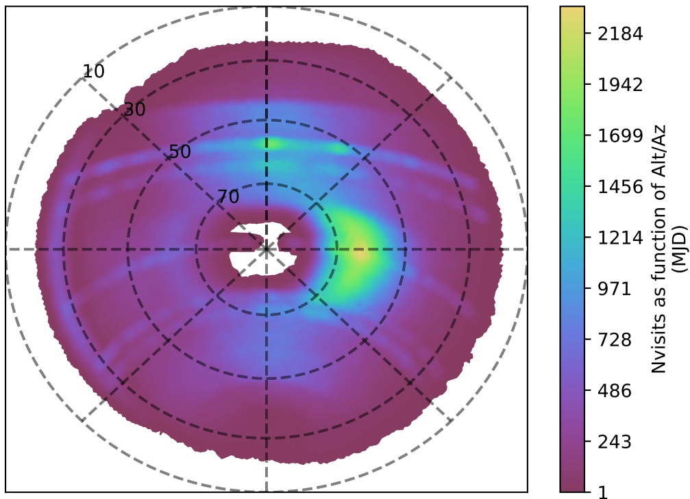
ddf_loaded_fl15_v3.4_10yrs r band: Nvisits as function of Alt/Az
