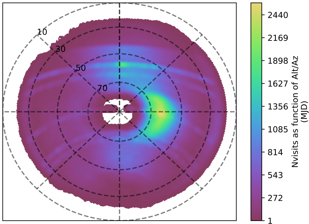
ddf_loaded_fl15_v3.4_10yrs i band: Nvisits as function of Alt/Az
