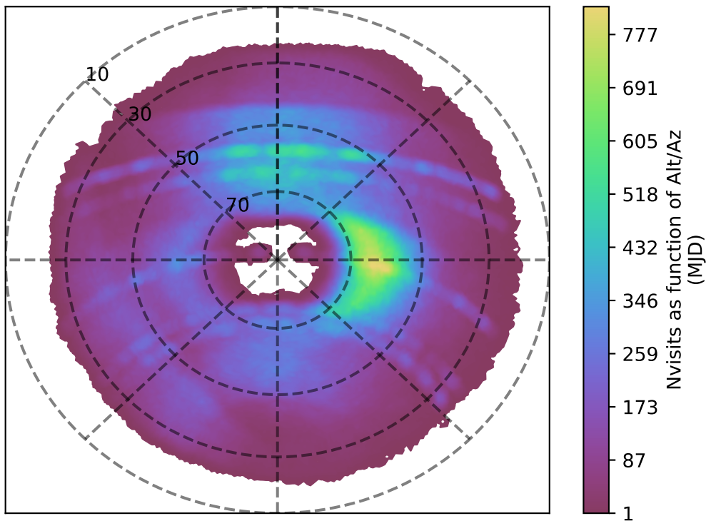
ddf_loaded_fl15_v3.4_10yrs g band: Nvisits as function of Alt/Az
