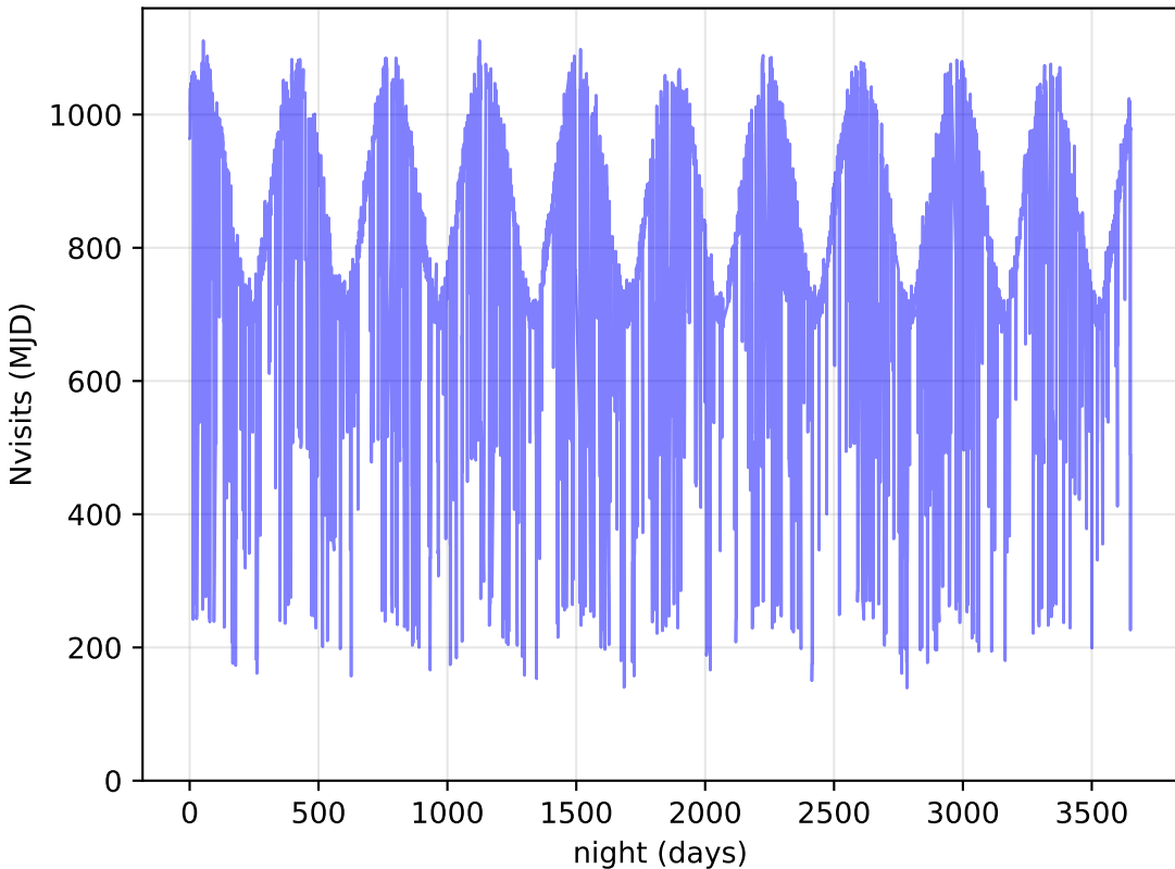
ddf_loaded_fl15_v3.4_10yrs All visits: Nvisits
