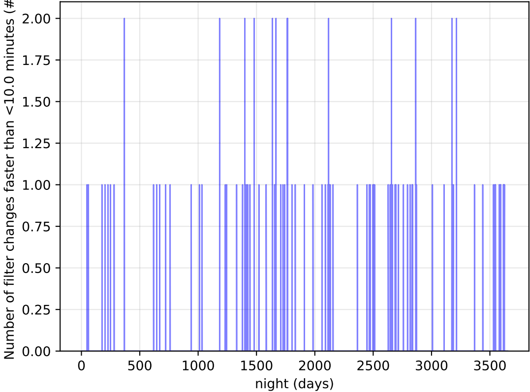
ddf_loaded_fl15_v3.4_10yrs Per Night: Number of filter changes faster than <10.0 minutes
