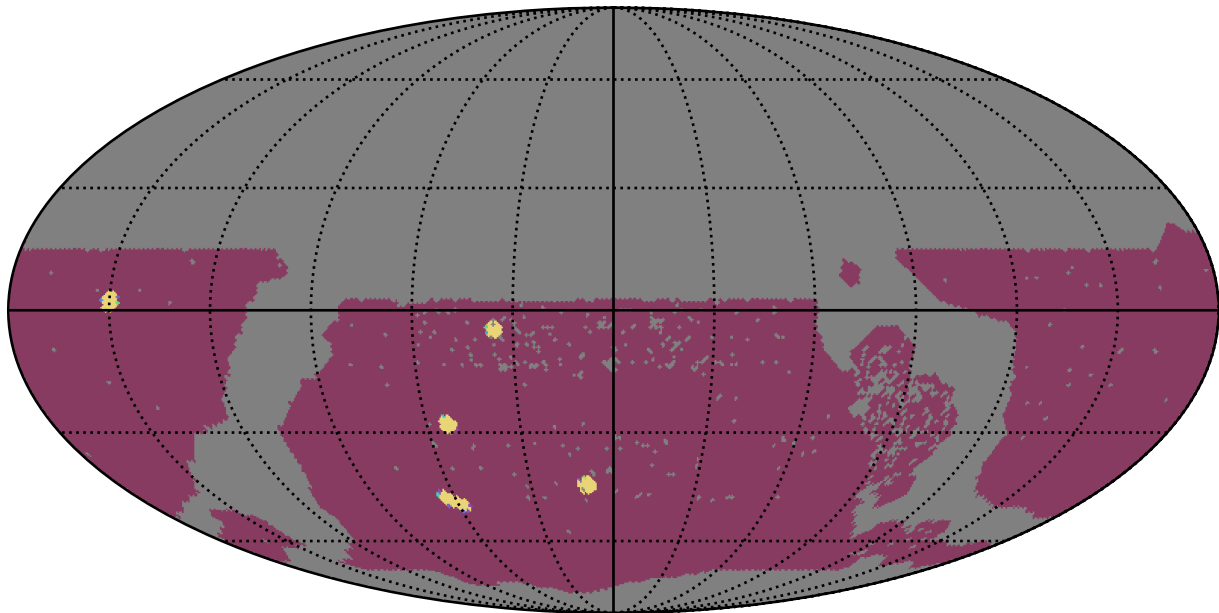
ddf_loaded_fl15_v3.4_10yrs WFD: NumberOfQuickRevisits
