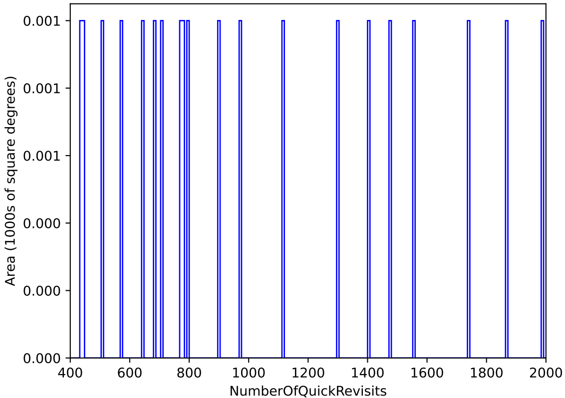
ddf_loaded_fl15_v3.4_10yrs WFD: NumberOfQuickRevisits
