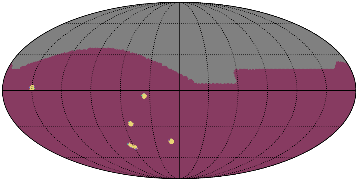
ddf_loaded_fl15_v3.4_10yrs All sky: NumberOfQuickRevisits
