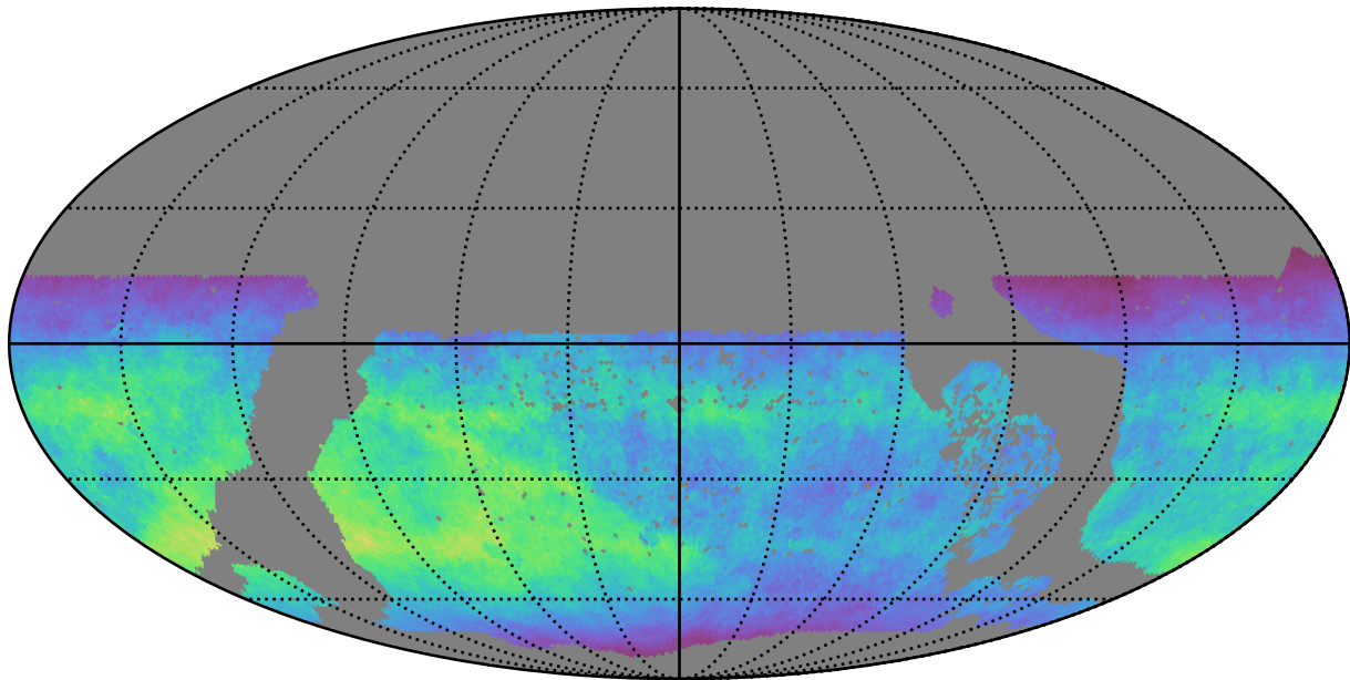
ddf_loaded_fl15_v3.4_10yrs WFD z band: Normalized Teff
