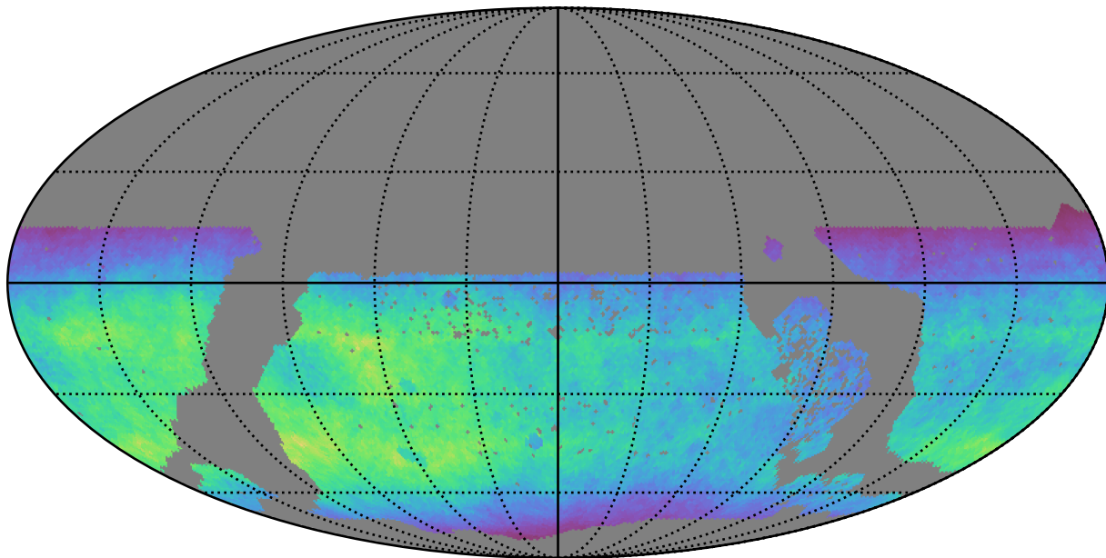
ddf_loaded_fl15_v3.4_10yrs WFD y band: Normalized Teff
