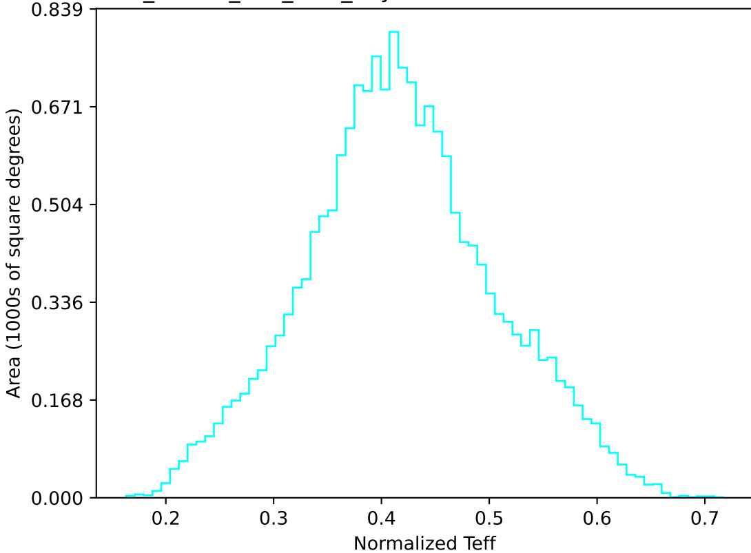
ddf_loaded_fl15_v3.4_10yrs WFD u band: Normalized Teff
