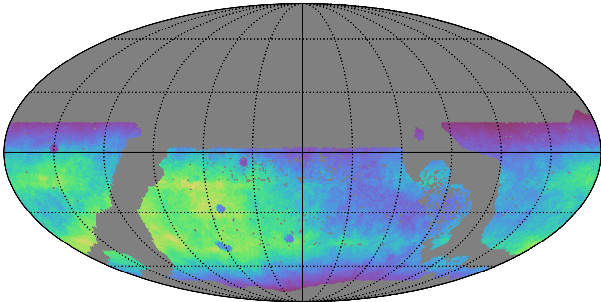
ddf_loaded_fl15_v3.4_10yrs WFD r band: Normalized Teff
