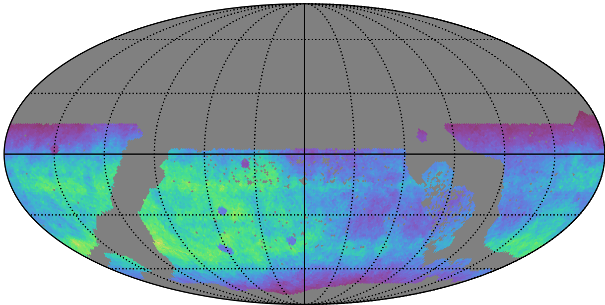
ddf_loaded_fl15_v3.4_10yrs WFD g band: Normalized Teff
