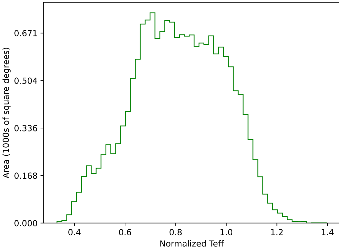
ddf_loaded_fl15_v3.4_10yrs WFD g band: Normalized Teff
