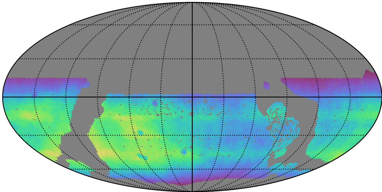
ddf_loaded_fl15_v3.4_10yrs WFD all bands: Normalized Teff
