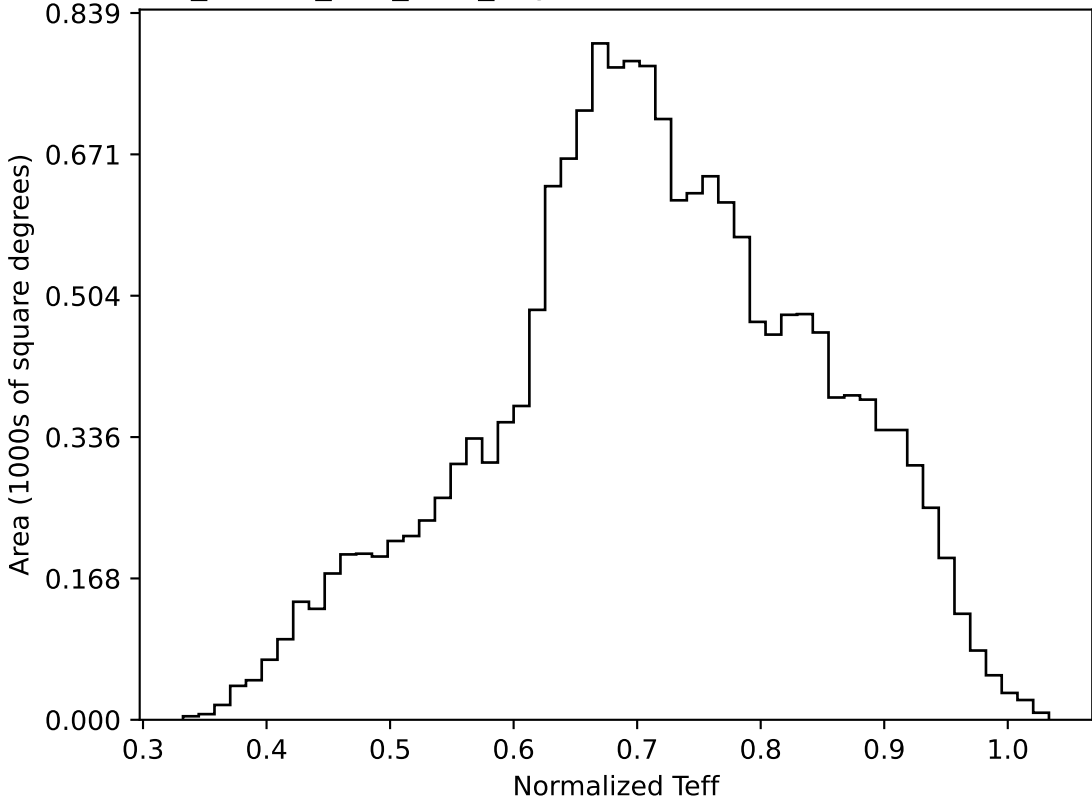
ddf_loaded_fl15_v3.4_10yrs WFD all bands: Normalized Teff
