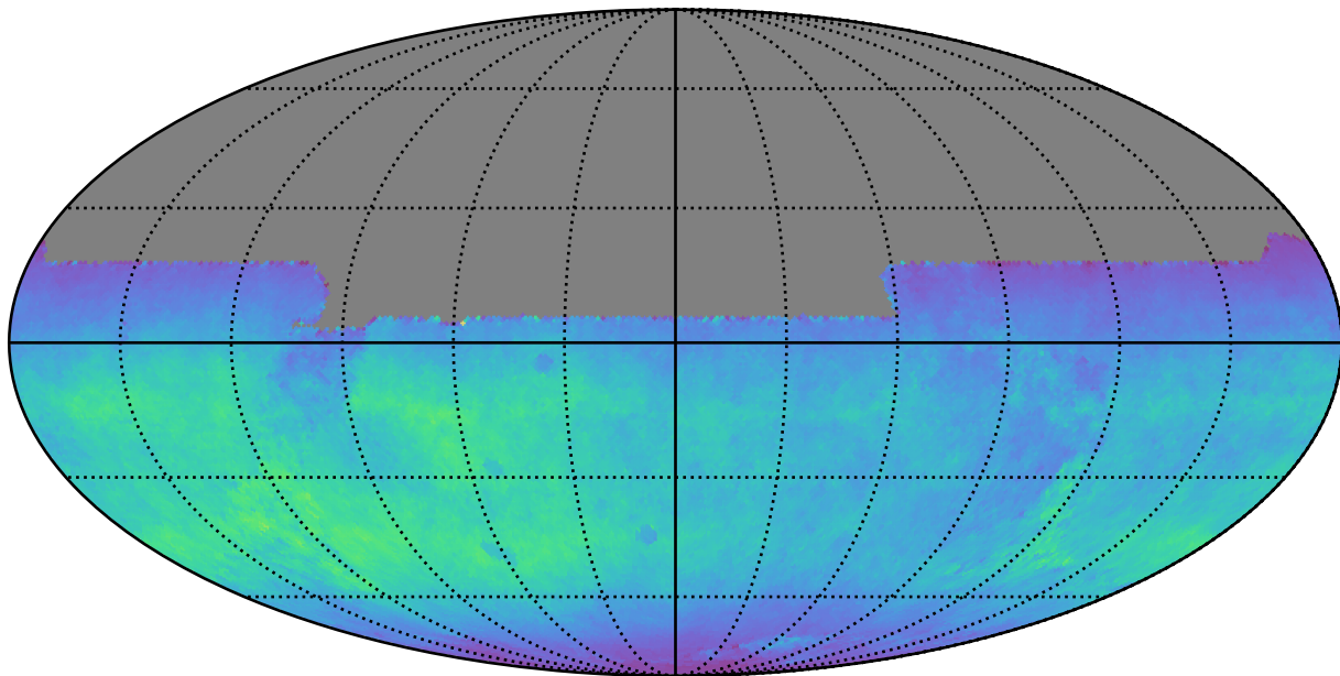
ddf_loaded_fl15_v3.4_10yrs All sky y band: Normalized Teff
