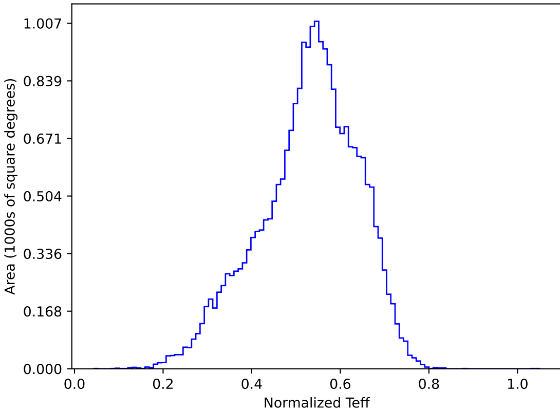
ddf_loaded_fl15_v3.4_10yrs All sky y band: Normalized Teff
