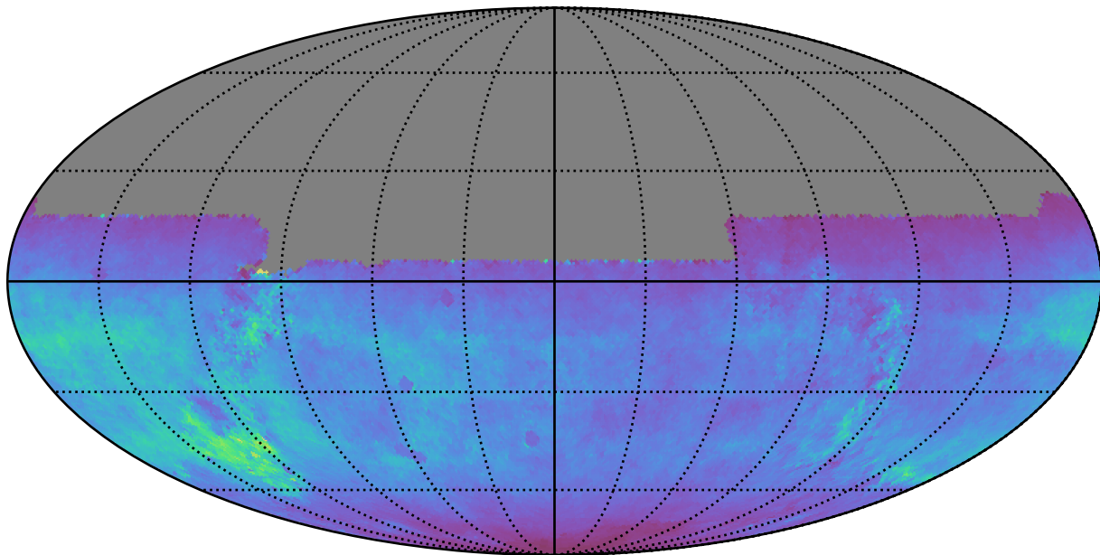
ddf_loaded_fl15_v3.4_10yrs All sky u band: Normalized Teff
