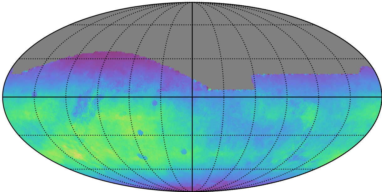
ddf_loaded_fl15_v3.4_10yrs All sky r band: Normalized Teff
