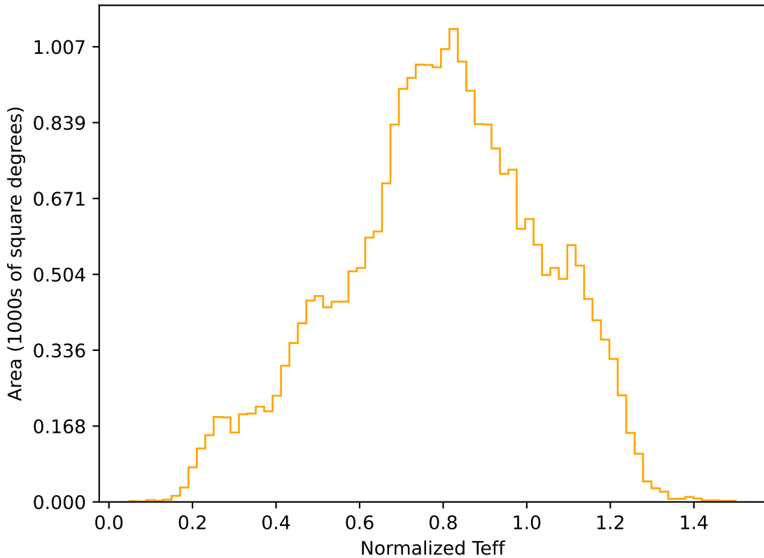
ddf_loaded_fl15_v3.4_10yrs All sky r band: Normalized Teff
