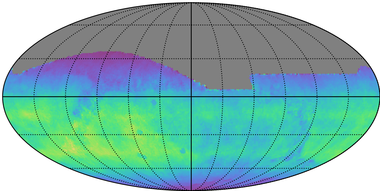
ddf_loaded_fl15_v3.4_10yrs All sky i band: Normalized Teff
