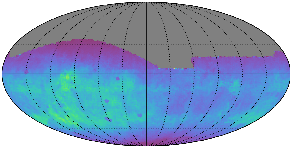
ddf_loaded_fl15_v3.4_10yrs All sky g band: Normalized Teff
