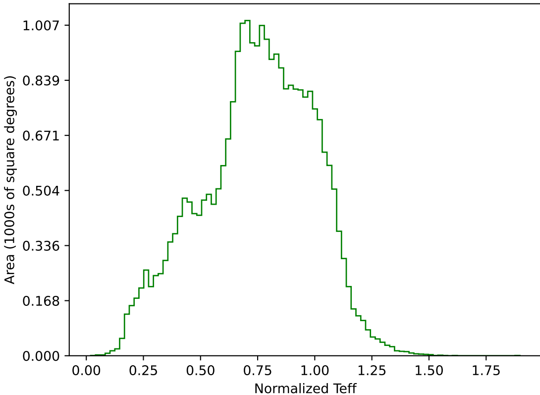
ddf_loaded_fl15_v3.4_10yrs All sky g band: Normalized Teff
