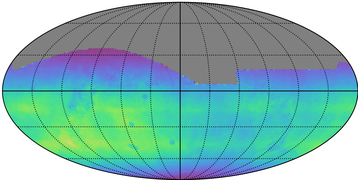
ddf_loaded_fl15_v3.4_10yrs All sky all bands: Normalized Teff
