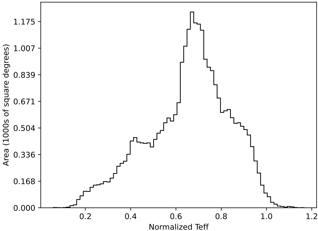
ddf_loaded_fl15_v3.4_10yrs All sky all bands: Normalized Teff
