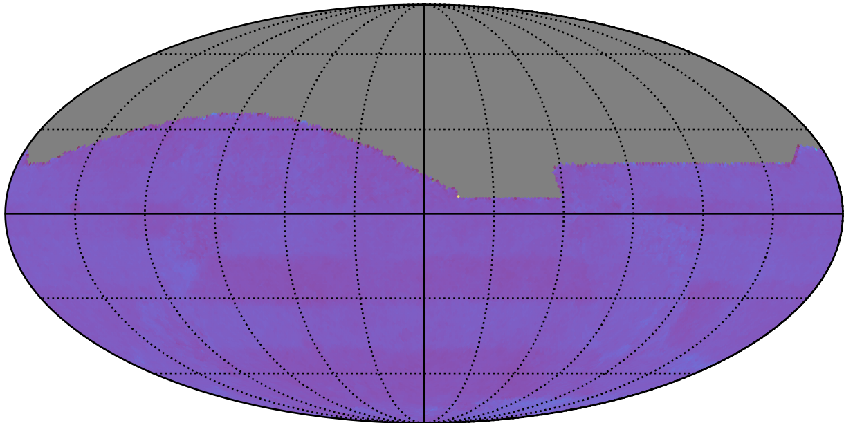
ddf_loaded_fl15_v3.4_10yrs All sky: Normalized Proper Motion Uncert @ 24.0
