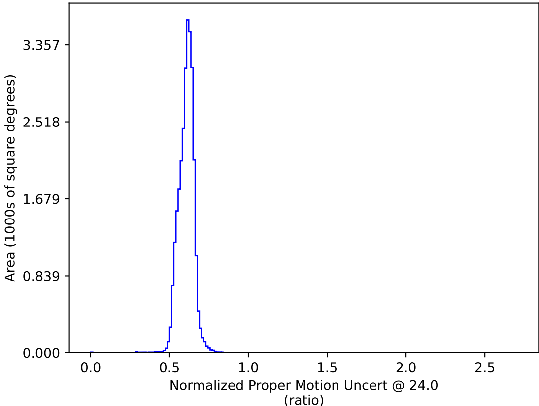
ddf_loaded_fl15_v3.4_10yrs All sky: Normalized Proper Motion Uncert @ 24.0
