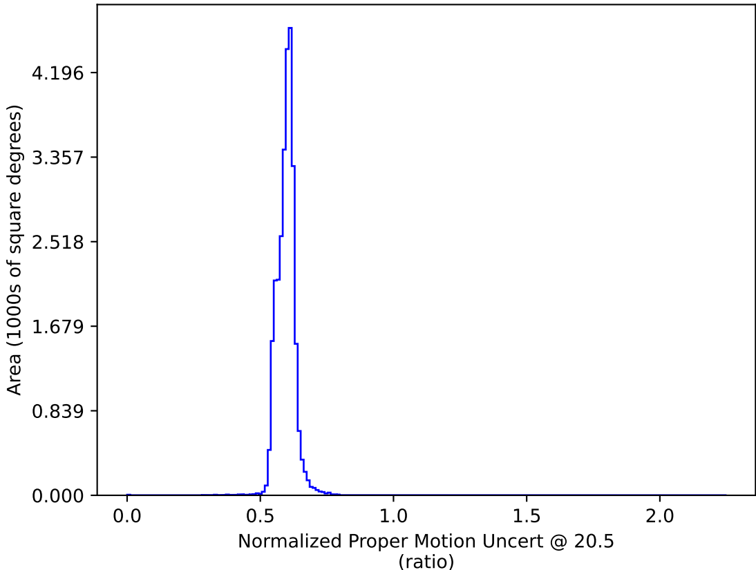
ddf_loaded_fl15_v3.4_10yrs All sky: Normalized Proper Motion Uncert @ 20.5
