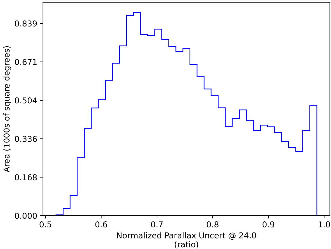
ddf_loaded_fl15_v3.4_10yrs WFD: Normalized Parallax Uncert @ 24.0
