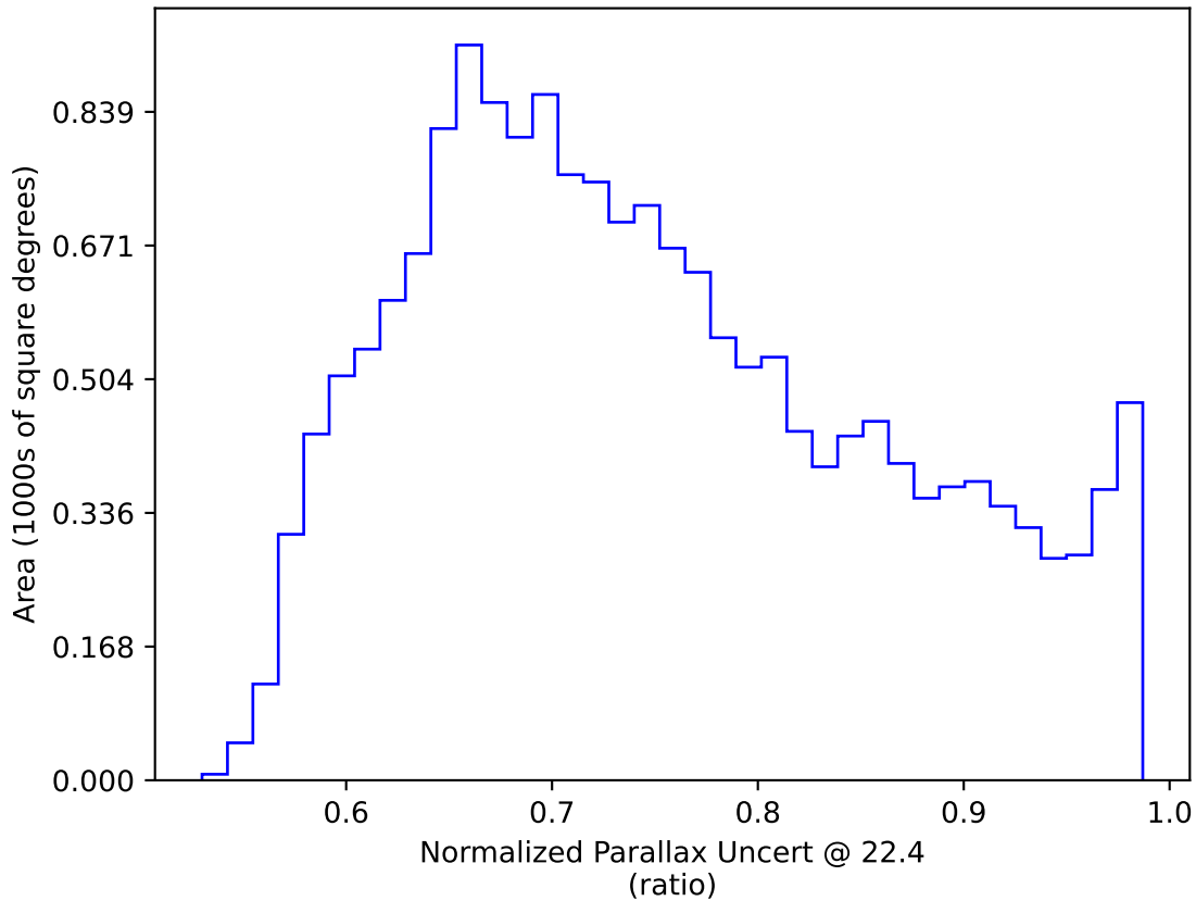
ddf_loaded_fl15_v3.4_10yrs WFD: Normalized Parallax Uncert @ 22.4
