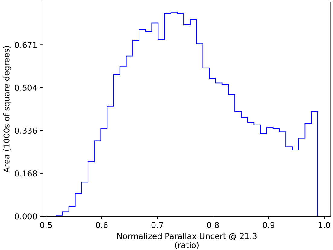
ddf_loaded_fl15_v3.4_10yrs WFD y band only: Normalized Parallax Uncert @ 21.3
