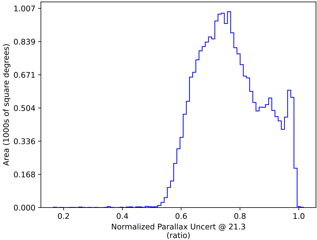
ddf_loaded_fl15_v3.4_10yrs All sky y band only: Normalized Parallax Uncert @ 21.3
