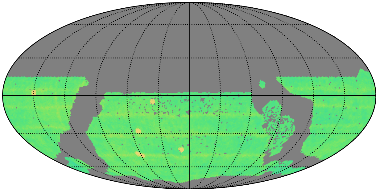
ddf_loaded_fl15_v3.4_10yrs WFD all bands: N Unique Nights
