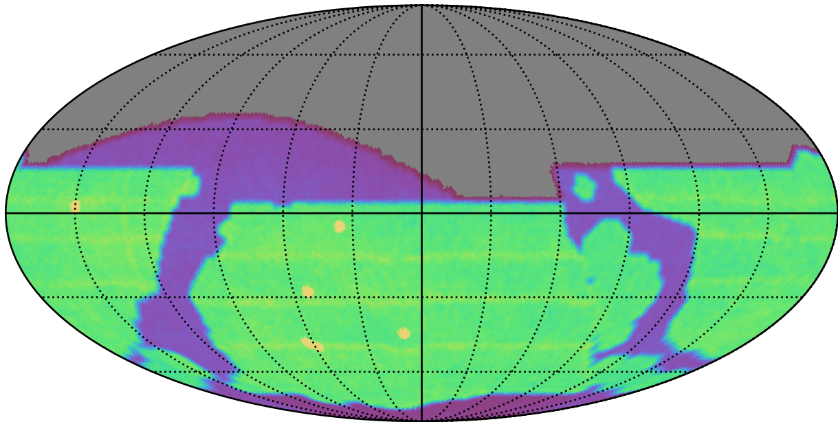
ddf_loaded_fl15_v3.4_10yrs All sky all bands: N Unique Nights
