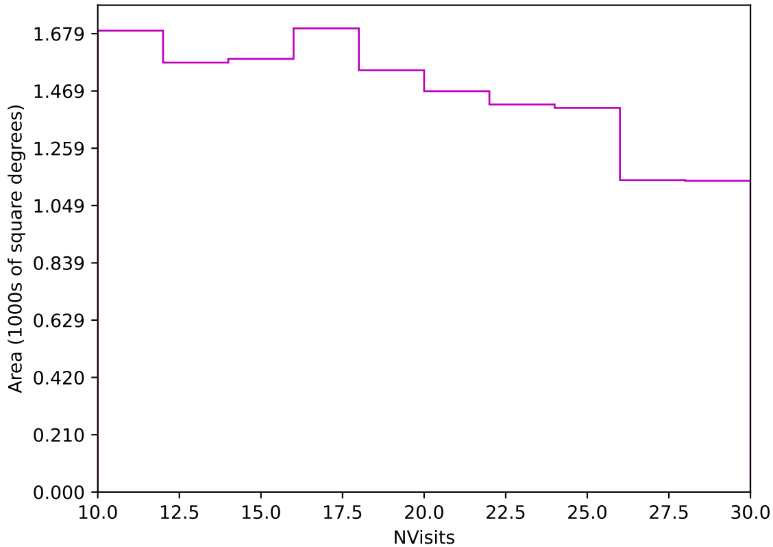
ddf_loaded_fl15_v3.4_10yrs Yr 3-4 z band: NVisits
