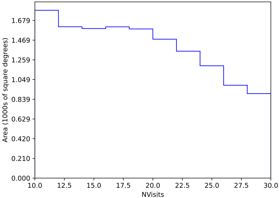
ddf_loaded_fl15_v3.4_10yrs Yr 3-4 y band: NVisits
