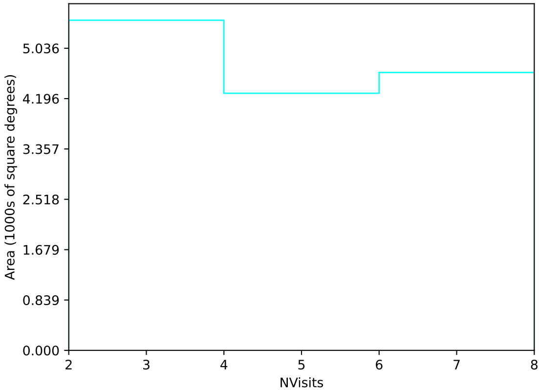
ddf_loaded_fl15_v3.4_10yrs Yr 3-4 u band: NVisits
