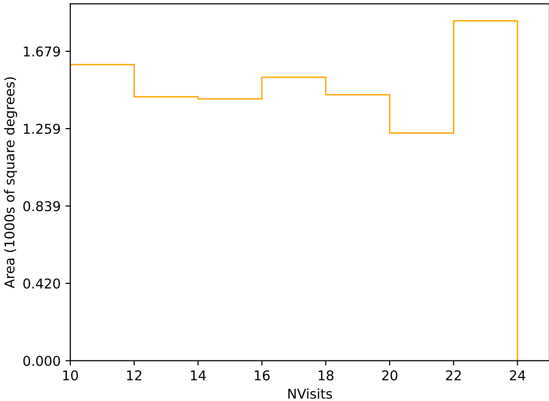
ddf_loaded_fl15_v3.4_10yrs Yr 3-4 r band: NVisits
