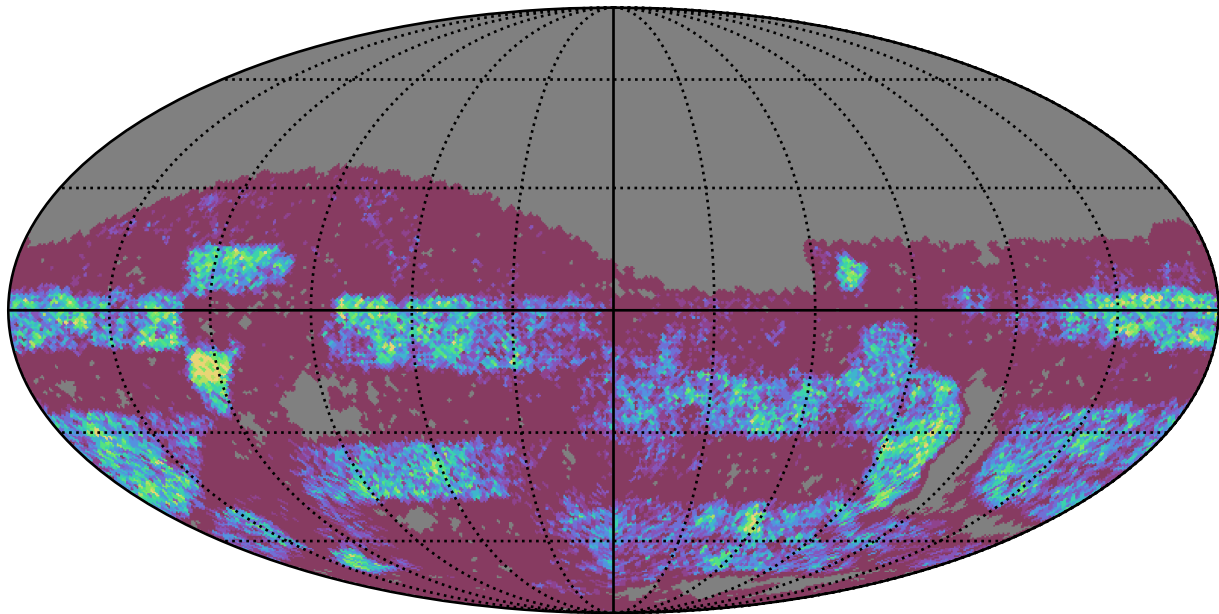
ddf_loaded_fl15_v3.4_10yrs Yr 3-4 g band: NVisits
