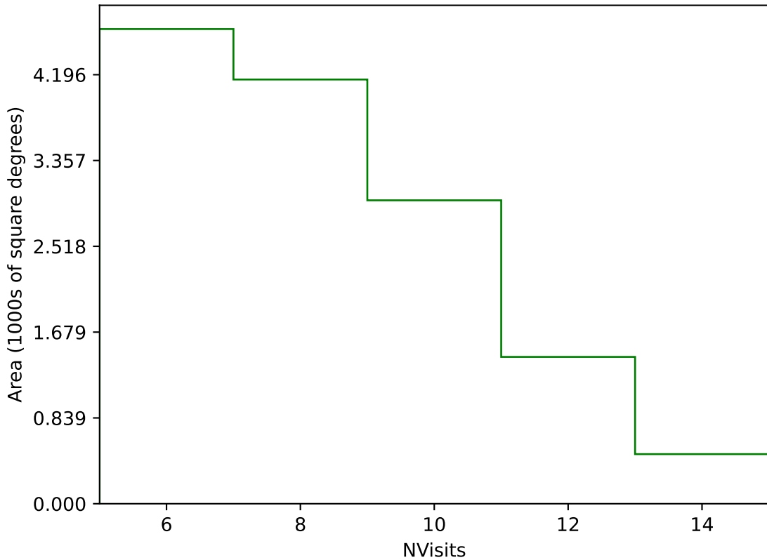
ddf_loaded_fl15_v3.4_10yrs Yr 3-4 g band: NVisits
