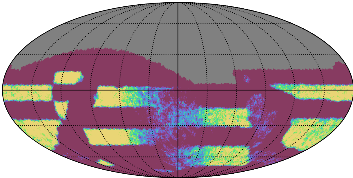
ddf_loaded_fl15_v3.4_10yrs Yr 3-4 all bands: NVisits
